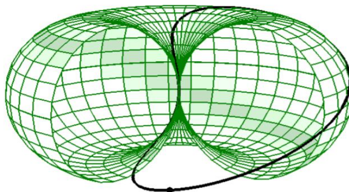
Fig. 1. The univon model composed of a superluminal primordial information quantum (spring). The mathematical horn torus surface on which the spring travels is cut away to show the interior. The black closed curve on the surface of the horn torus is the trajectory of the univon’s spring (indicated by the black dot.)
